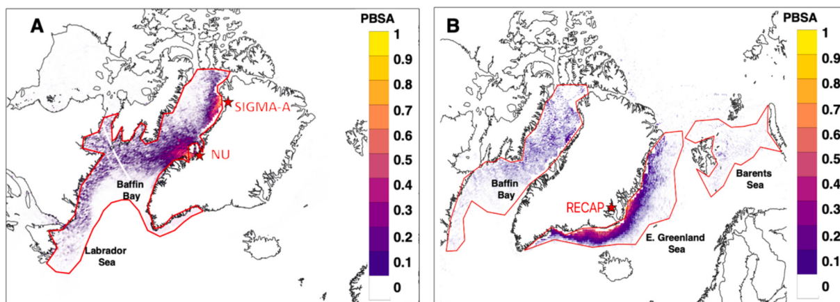
Fig. 2. The Potential Bromine Source Area (PBSA) of SIGMA-A, NU, and RECAP ice cores in the recent period (1984-onward). (A) The red contour delineates the combined PBSA of western Greenland ice cores (averaged and normalized for MAM 1984–2016 (SIGMA-A) and 1984–2013 (NU)). (B) Similarly, the RECAP's PBSA averaged and normalized over MAM 1984–2012. Among the three sectors identified, the East Greenland Sea accounts for most of the potential bromine contribution (~90 %), compared to Barents Sea and central Baffin Bay (~10 %).
