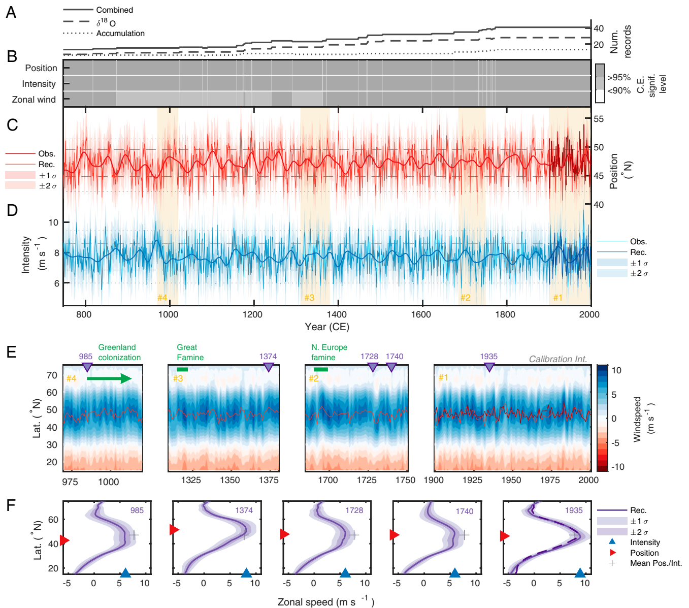
Fig. 3. Skillful reconstruction of the North Atlantic zonal wind profile during the last millennium. (A) Availability of Greenland \delta^{18}\text{O} and annually accumulated snowfall ice-core records over time. (B) Coefficient of efficiency (C.E.) significance levels for NAJ position, intensity, and the North Atlantic zonal wind profile for all nested models. Note that all nests have C.E. values greater than 0, signifying skill above climatology in the reconstruction. (C) NAJ position (red) and (D) intensity (blue) derived from the North Atlantic zonal wind profile reconstruction. The dark lines show NAJ position and intensity from the NOAA20C reanalysis, and the bold smooth lines show 30-y low-pass-filtered time series. Underlying dashed and dotted levels show the \pm 1\sigma range and the middle 95% range, respectively. (E) Hovmöller diagrams of the North Atlantic zonal wind profile for four selected time periods; note that observed and reconstructed NAJ positions are illuminated as dark (right panel) and light (all panels) red lines, respectively. Purple arrows at top of E denote years shown in F. (F) Selected annual snapshots of the North Atlantic zonal wind profile, as discussed in the text. All results shown are calibrated to the NOAA20C reanalysis (23) over 1900 to 2000 CE.
